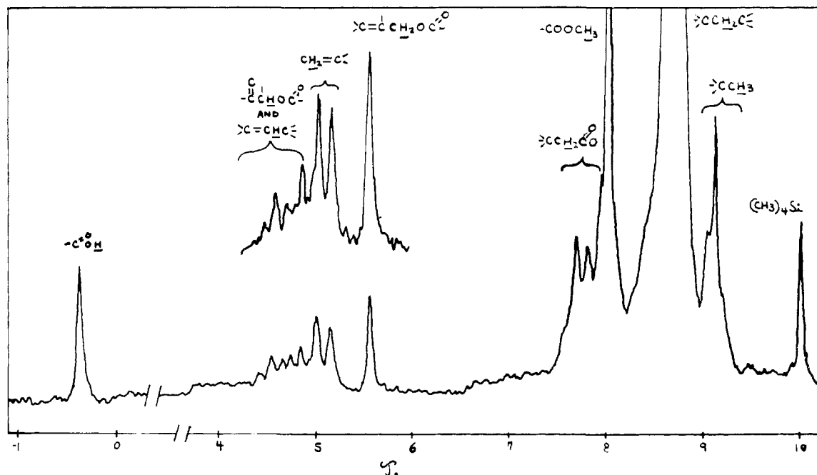
Fig. 3.—Nuclear magnetic resonance spectrum of mixture C.
