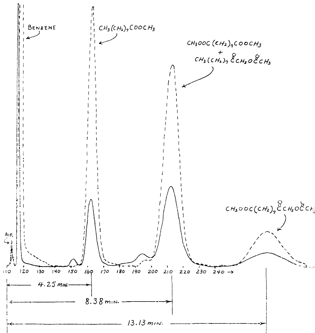
Fig. 1. —Gas chromatograms of compounds III, IV, V and VI ( R = CH_3 ): —, from oxidation of mixture C; ----, from a prepared mixture of authentic compounds.
